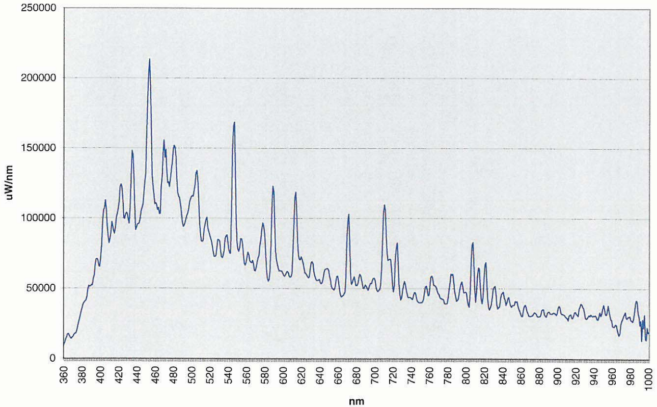
Radiant Plot
