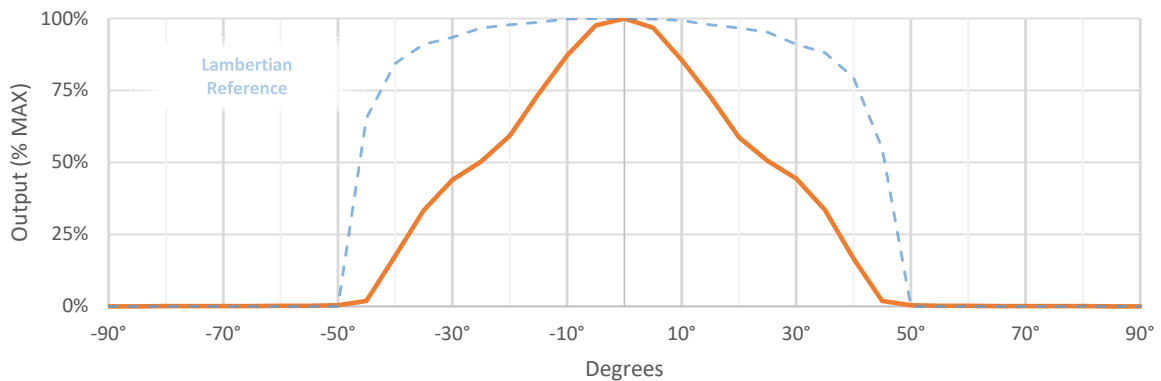
Beam Pattern Angular Distribution
