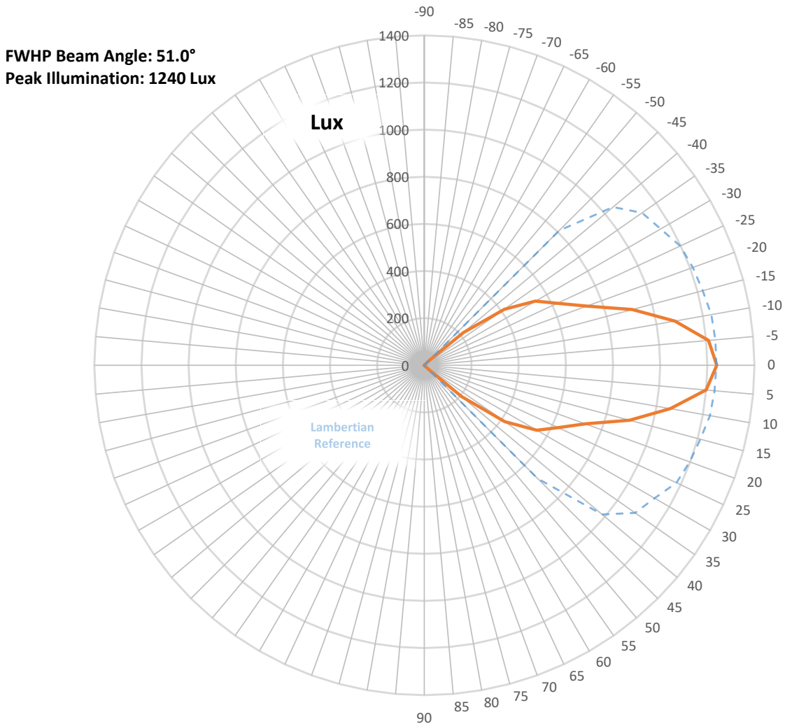
Beam Pattern Angular Distribution
